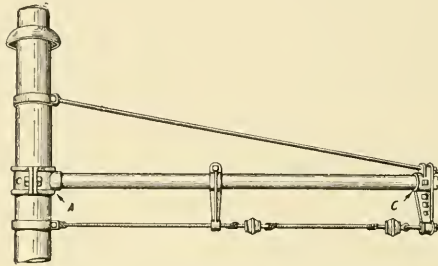
Fig. 196. Bracket Used on Metal Poles
